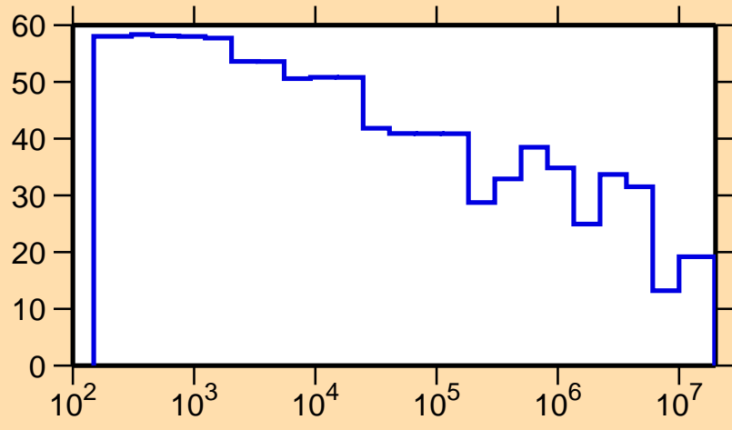
\Delta\sigma/\sigma vs. E for ^{193}\text{Tl}(n,el.)
