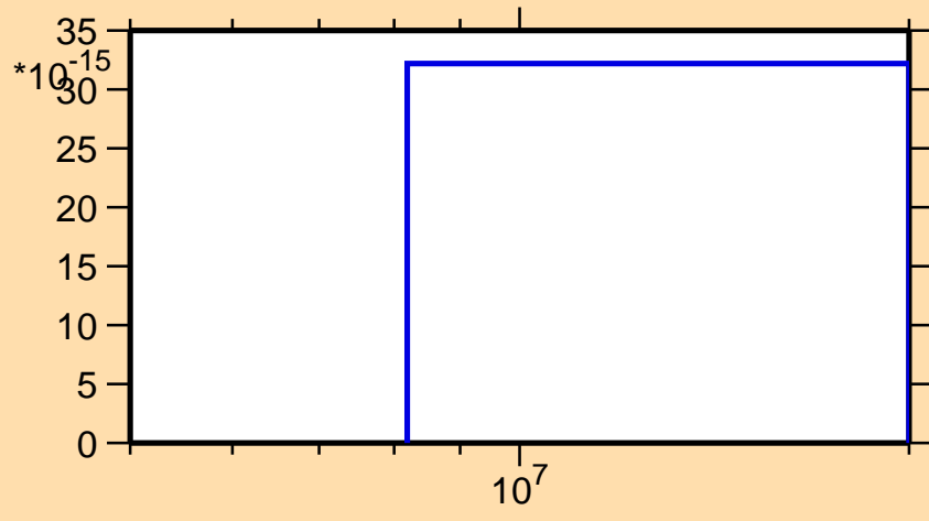
\sigma vs. E for ^{193}\text{Tl}(n,3n\alpha)
