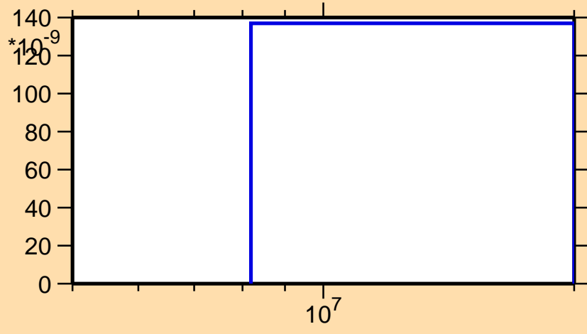
\sigma vs. E for ^{193}\text{Tl}(n,2n\alpha)
