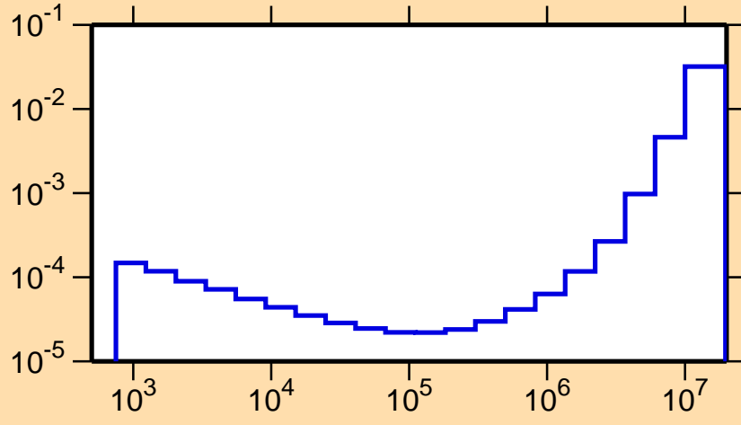
\sigma vs. E for ^{193}\text{Tl}(n,p)
