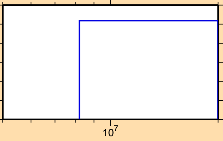
\sigma vs. E for ^{193}\text{Tl}(n,2n\alpha)
