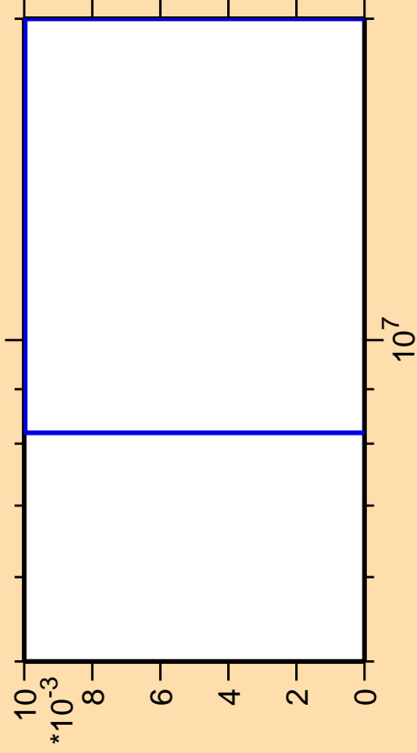
\Delta\sigma/\sigma vs. E for ^{193}\text{Tl}(n,3n\alpha)
