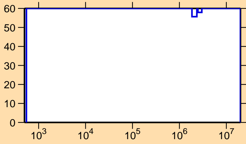
\Delta\sigma/\sigma vs. E for ^{193}\text{Tl}(n,n_1)
