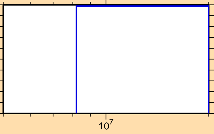
\sigma vs. E for ^{193}\text{Tl}(n,\text{He}3)
