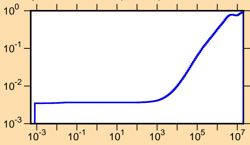
\mu vs. E for ^{194}\text{Tl}(\text{mt251})
