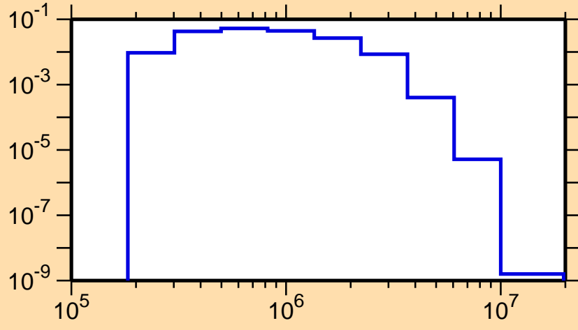
\sigma vs. E for ^{194}\text{Tl}(n,n_3)
