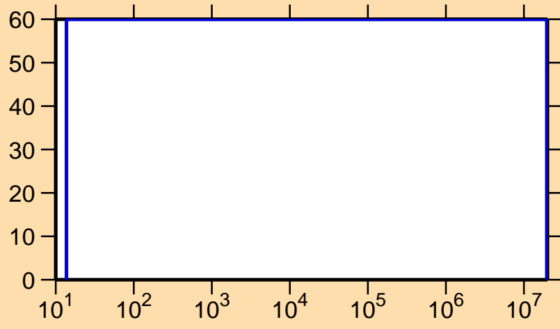
\Delta\sigma/\sigma vs. E for ^{194}\text{Tl}(n,p)
