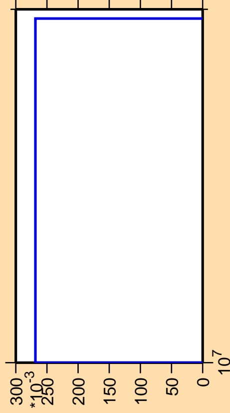
\Delta\sigma/\sigma vs. E for ^{194}\text{Tl} (mt 34)
