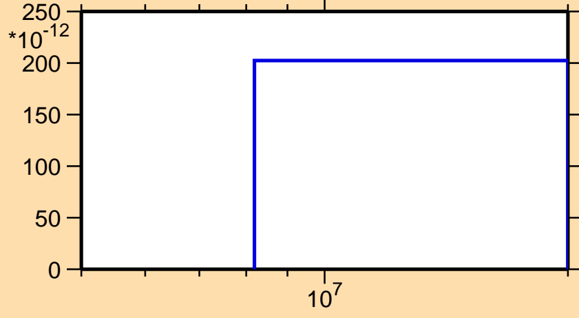
\sigma vs. E for ^{194}\text{Tl}(n,nt)
