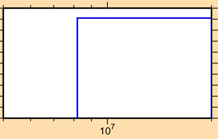
\sigma vs. E for ^{194}\text{Tl}(n,\text{He}3)
