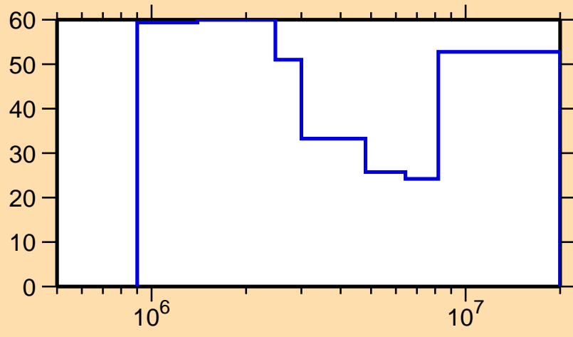
\Delta\sigma/\sigma vs. E for ^{194}\text{Tl}(n,n\text{cont.})
