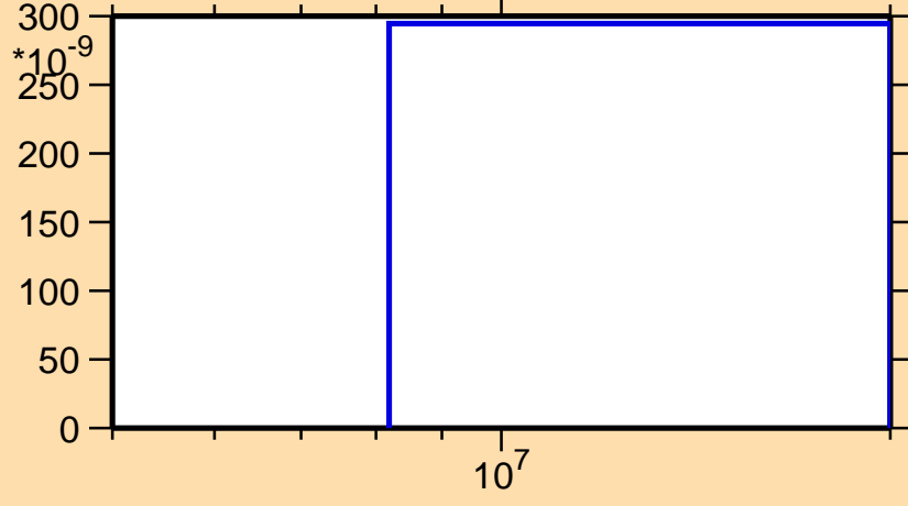
\sigma vs. E for ^{194}\text{Tl}(n,nd)
