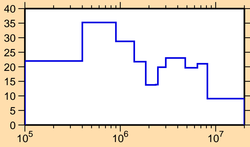
\Delta\sigma/\sigma vs. E for ^{194}\text{Tl}(n,\text{tot.})
