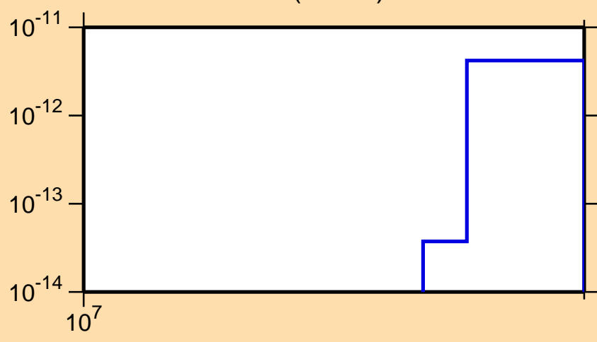
\sigma vs. E for ^{194}\text{Tl} (mt 34)
