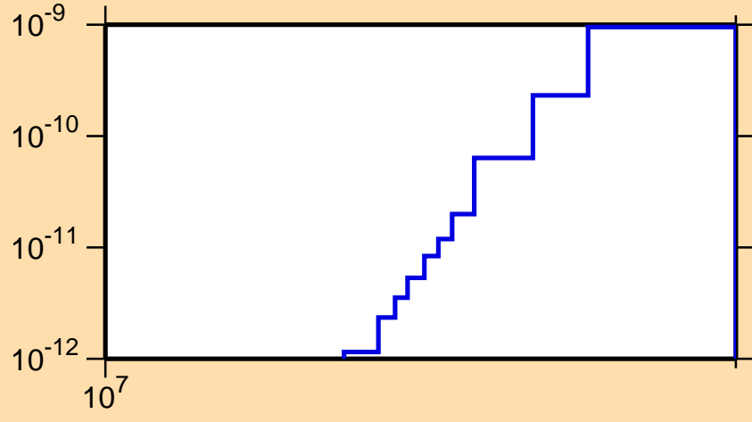
\sigma vs. E for ^{194}\text{Tl}(\text{mt117})
