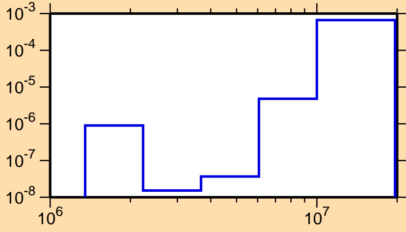
\sigma vs. E for ^{194}\text{Tl}(n,n\alpha)
