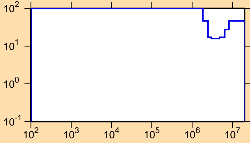
\Delta\sigma/\sigma vs. E for ^{194}\text{Tl}(n,ncont.)
