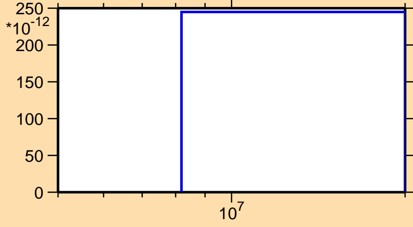
\sigma vs. E for ^{194}\text{Tl} (mt 45)
