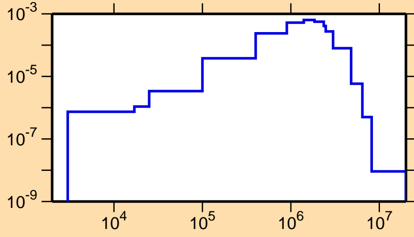
\sigma vs. E for ^{194}\text{Tl}(n,n_1)
