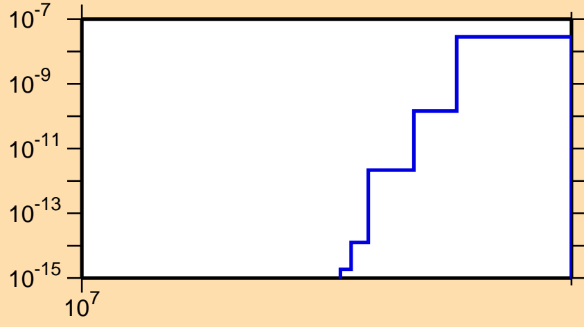
\sigma vs. E for ^{195}\text{Tl}(n,nt)
