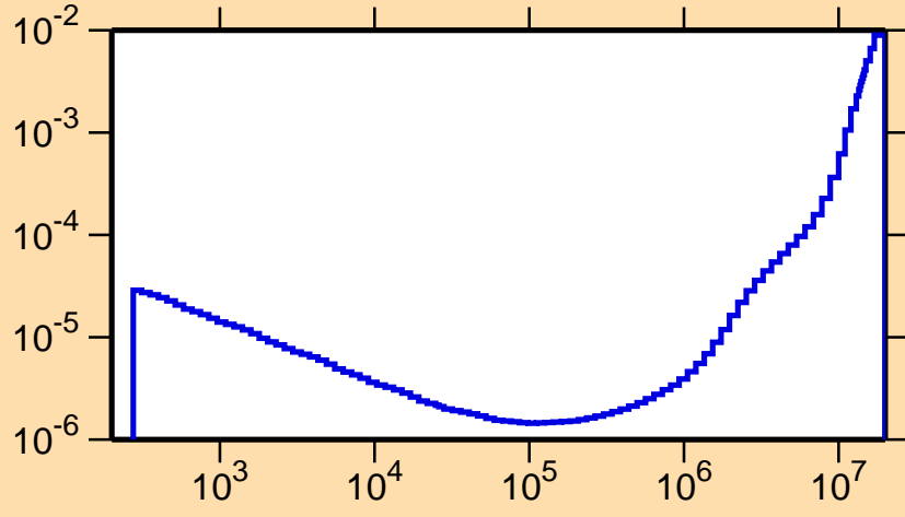
\sigma vs. E for ^{195}\text{Tl}(n,\alpha)
