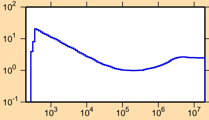
\sigma vs. E for ^{195}\text{Tl}(n,\text{nonel.})
