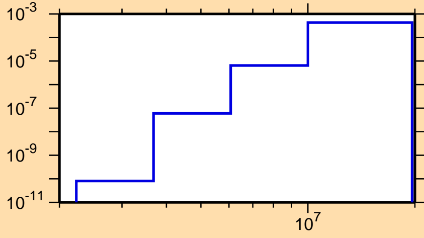
\sigma vs. E for ^{195}\text{Tl}(n,n\alpha)
