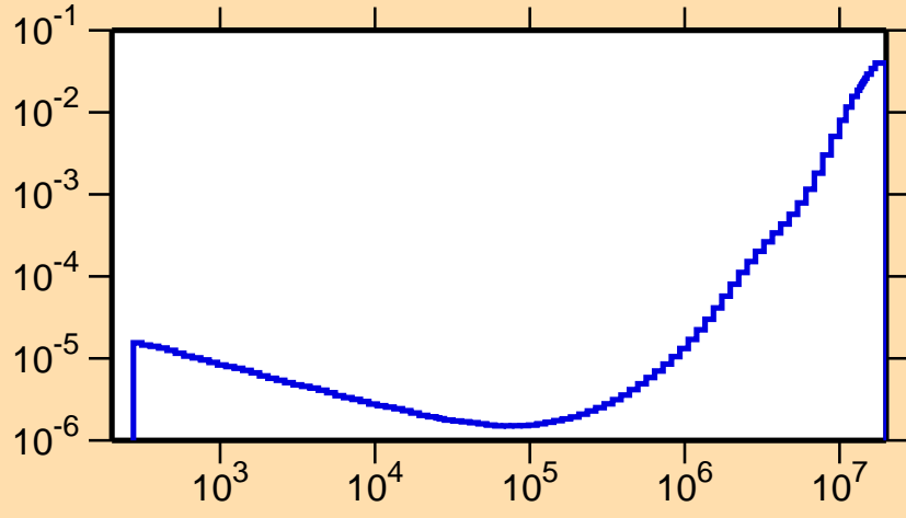
\sigma vs. E for ^{195}\text{Tl}(n,p)
