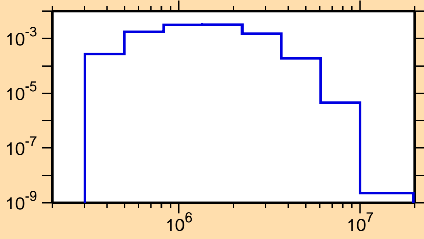
\sigma vs. E for ^{195}\text{Tl}(n,n_4)
