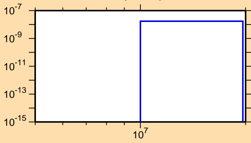
\sigma vs. E for ^{195}\text{Tl}(n,2n\alpha)
