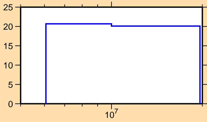
\Delta\sigma/\sigma vs. E for ^{195}\text{Tl}(n,\text{nonel.})
