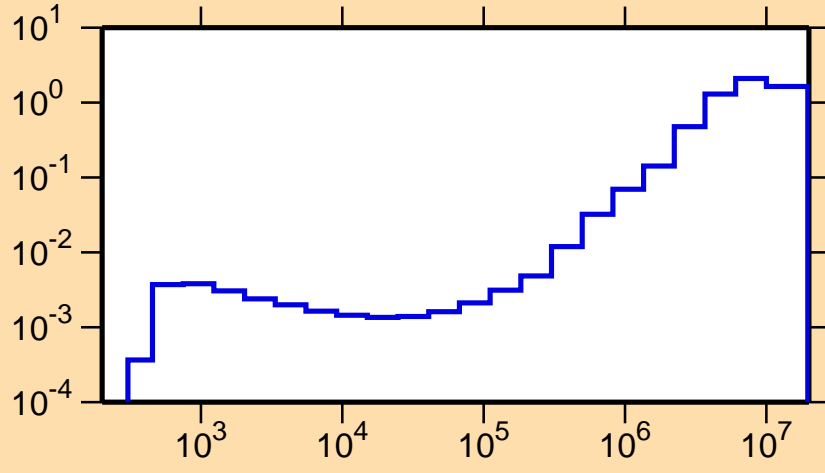
\sigma vs. E for ^{195}\text{Tl}(n,\text{inel.})
