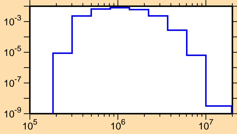
\sigma vs. E for ^{195}\text{Tl}(n,n_3)
