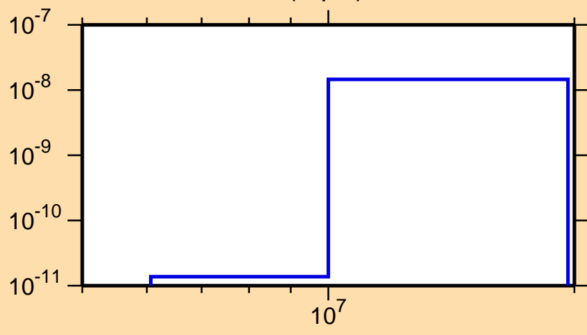
\sigma vs. E for ^{195}\text{Tl}(n,p\alpha)
