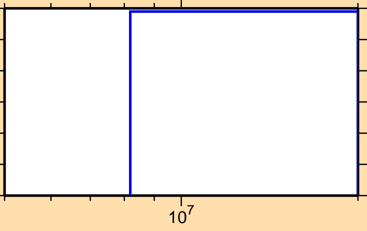
\sigma vs. E for ^{195}\text{Tl}(n,\text{nd})
