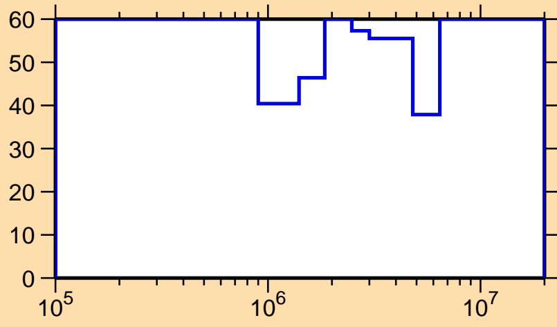
\Delta\sigma/\sigma vs. E for ^{195}\text{Tl}(n,n_1)
