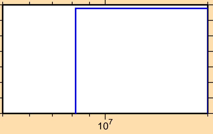
\sigma vs. E for ^{195}\text{Tl}(n,\text{He}3)
