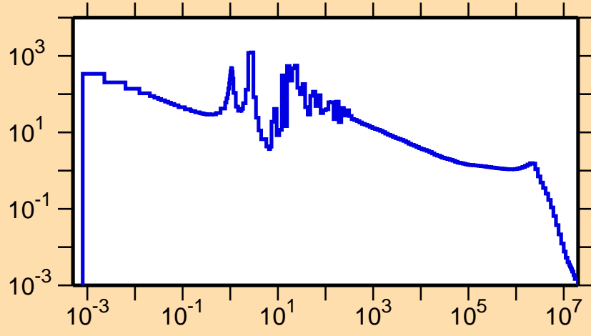
\sigma vs. E for ^{196}\text{Tl}(n,\gamma)
