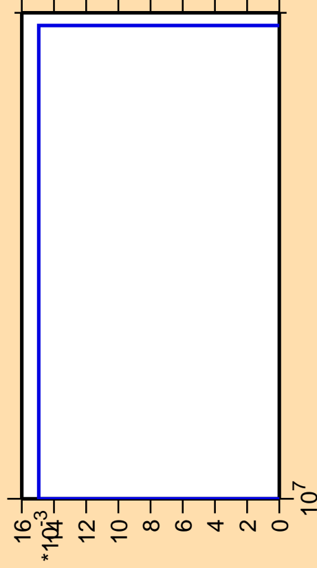
\Delta\sigma/\sigma vs. E for ^{196}\text{Tl}(n,pd)
