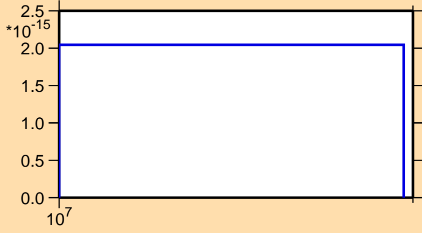
\sigma vs. E for ^{196}\text{Tl} (mt 34)
