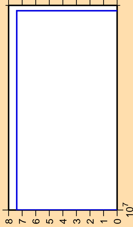
\Delta\sigma/\sigma vs. E for ^{196}\text{Tl}(\text{mt117})
