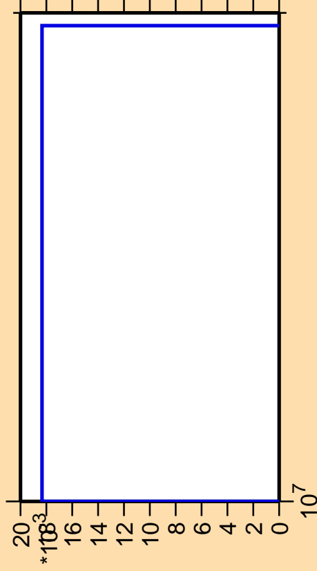
\Delta\sigma/\sigma vs. E for ^{196}\text{Tl} (mt 34)
