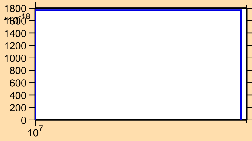
\sigma vs. E for ^{196}\text{Tl}(n,pd)
