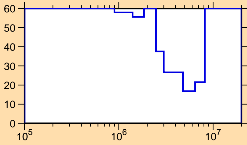
\Delta\sigma/\sigma vs. E for ^{196}\text{Tl}(n,n\text{cont.})
