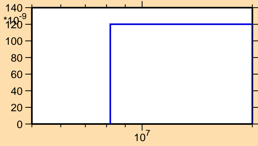
\sigma vs. E for ^{196}\text{Tl}(n,nd)
