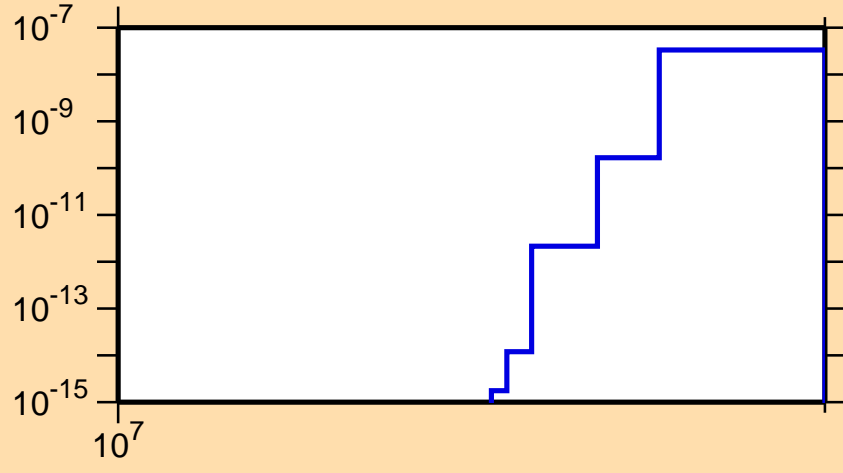
\sigma vs. E for ^{197}\text{Tl}(n,nt)
