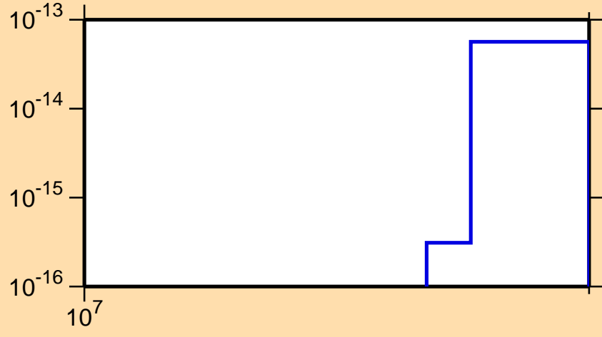
\sigma vs. E for ^{197}\text{Tl}(n,\text{pd})
