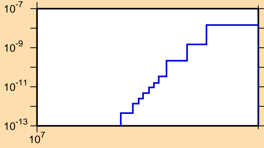
\sigma vs. E for ^{197}\text{Tl}(n,\text{He}3)
