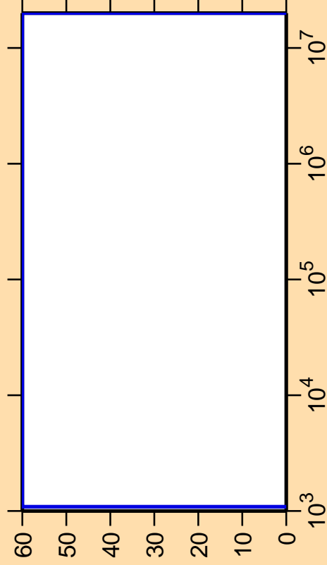
\Delta\sigma/\sigma vs. E for ^{197}\text{Tl}(n,\alpha)
