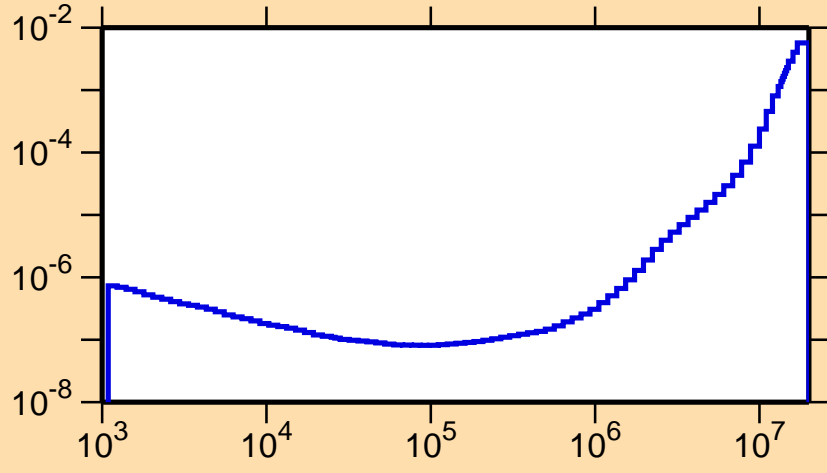
\sigma vs. E for ^{197}\text{Tl}(n,\alpha)
