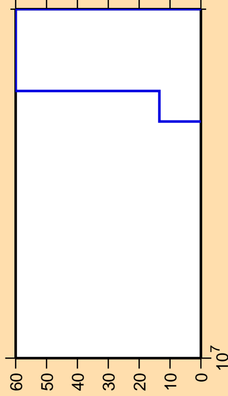
\Delta\sigma/\sigma vs. E for ^{197}\text{Tl} (mt 45)
