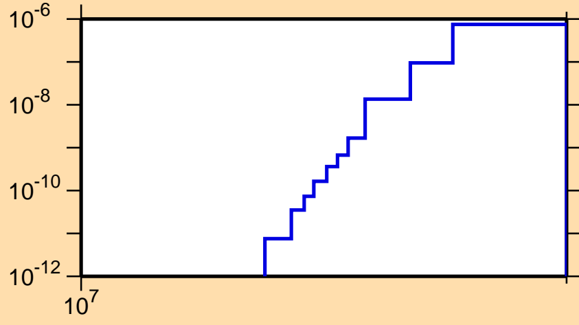
\sigma vs. E for ^{197}\text{Tl}(n,2n\alpha)
