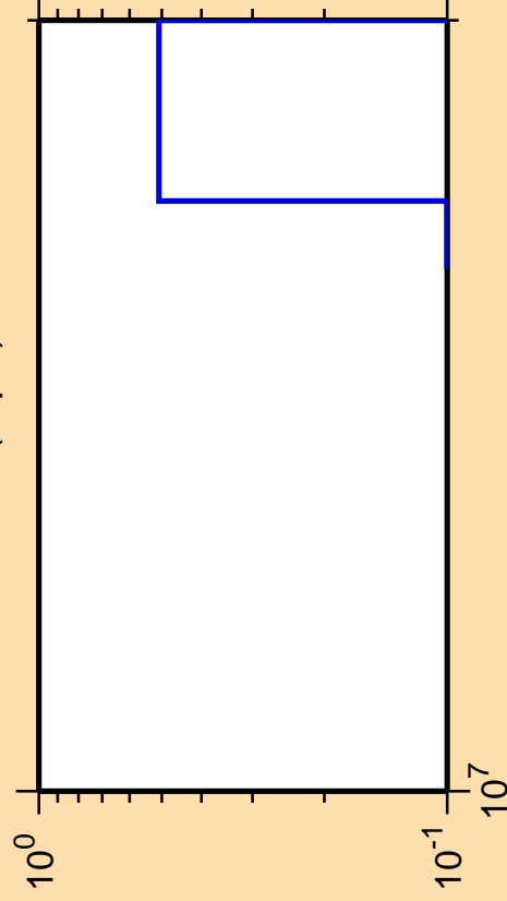
\Delta\sigma/\sigma vs. E for ^{197}\text{Tl}(n,\text{pd})
