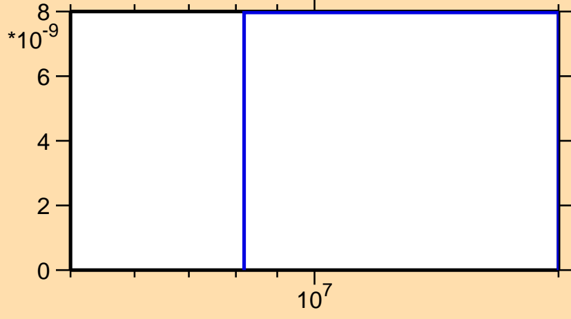
\sigma vs. E for ^{197}\text{Tl}(n,nd)
