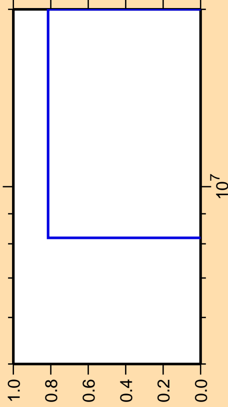
\Delta\sigma/\sigma vs. E for ^{197}\text{Tl}(\text{mt117})
