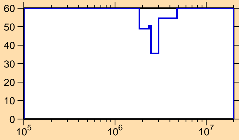
\Delta\sigma/\sigma vs. E for ^{197}\text{Tl}(n,n_1)
