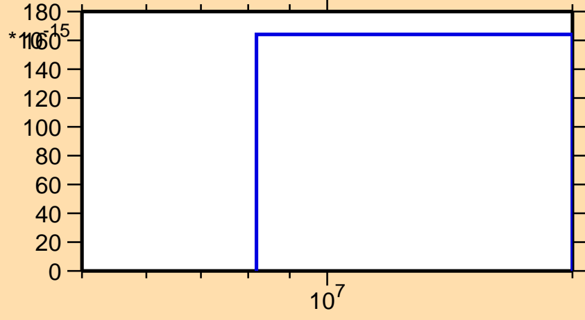
\sigma vs. E for ^{197}\text{Tl}(\text{mt117})
