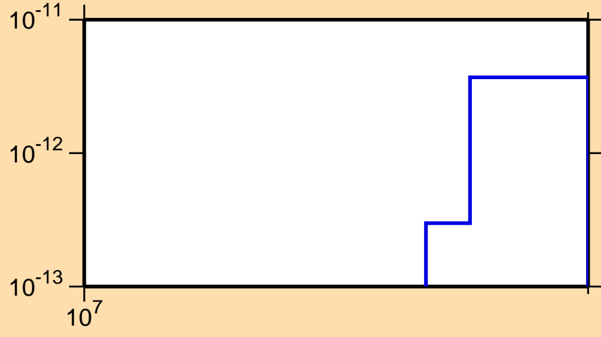
\sigma vs. E for ^{198}\text{Tl} (mt 45)
