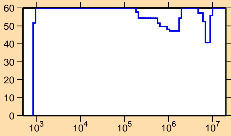
\Delta\sigma/\sigma vs. E for ^{198}\text{Tl}(n,\gamma)
