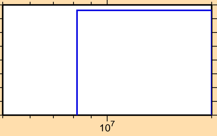
\sigma vs. E for ^{198}\text{Tl}(n,nt)
