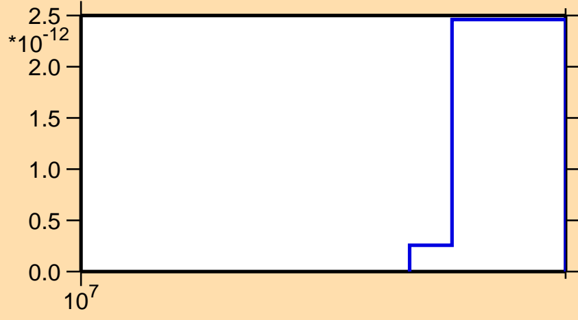
\sigma vs. E for ^{198}\text{Tl}(\text{mt117})
