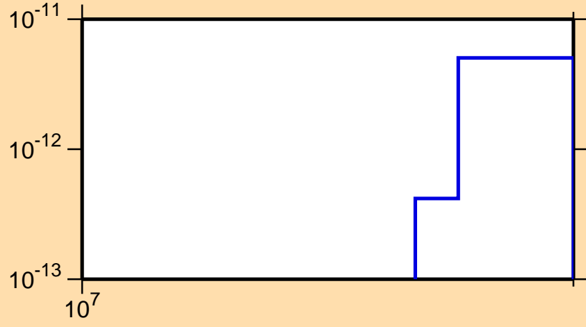
\sigma vs. E for ^{198}\text{Tl} (mt 45)
