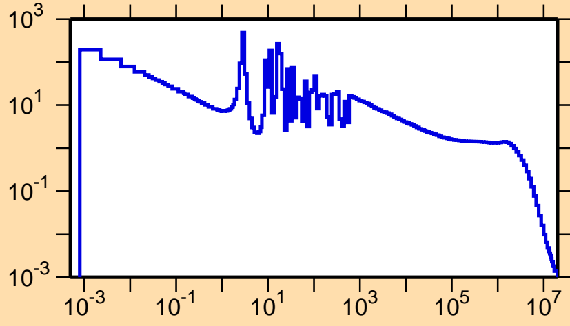
\sigma vs. E for ^{198}\text{Tl}(n,\gamma)
