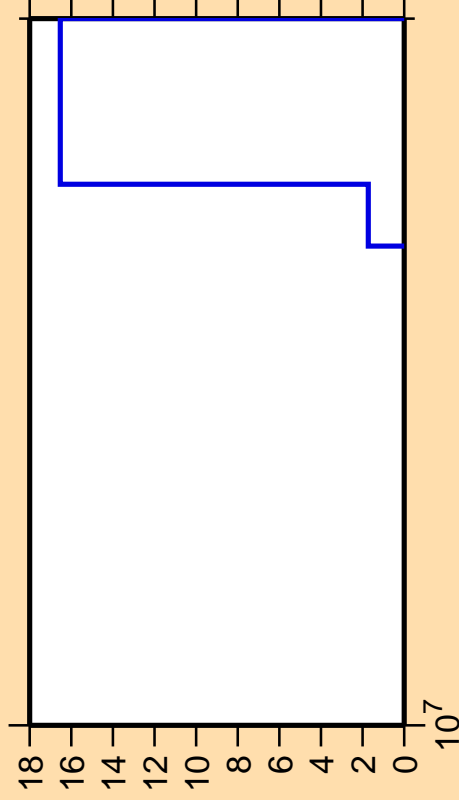
\Delta\sigma/\sigma vs. E for ^{198}\text{Tl}(\text{mt117})
