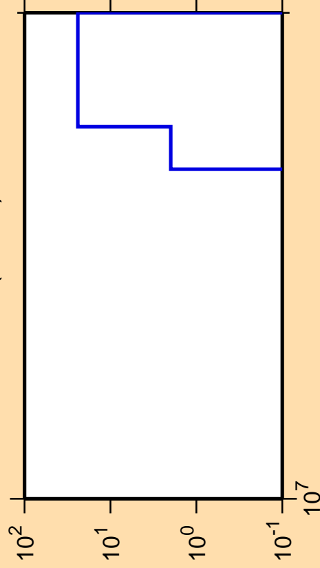
\Delta\sigma/\sigma vs. E for ^{198}\text{Tl} (mt 45)
