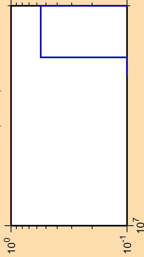
\Delta\sigma/\sigma vs. E for ^{198}\text{Tl} (mt 34)
