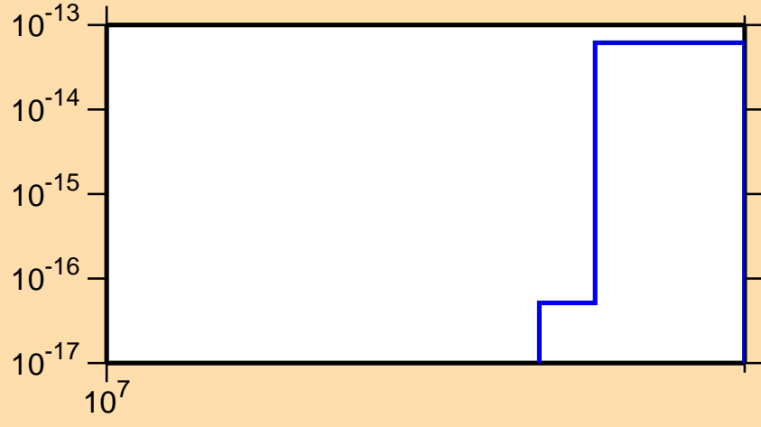
\sigma vs. E for ^{198}\text{Tl} (mt 34)
