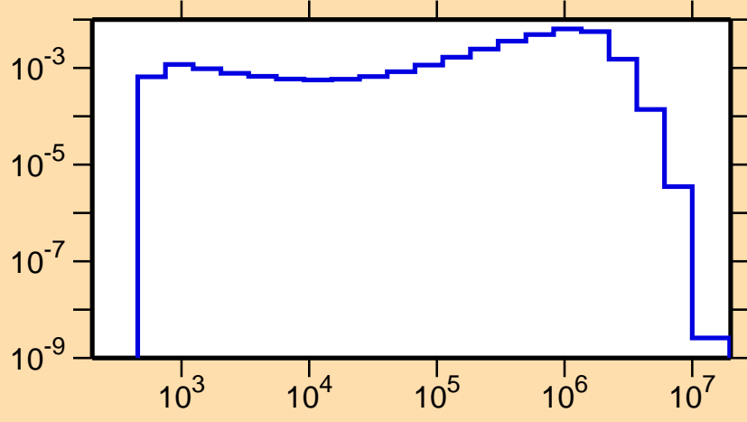
\sigma vs. E for ^{198}\text{Tl}(n,n_4)
