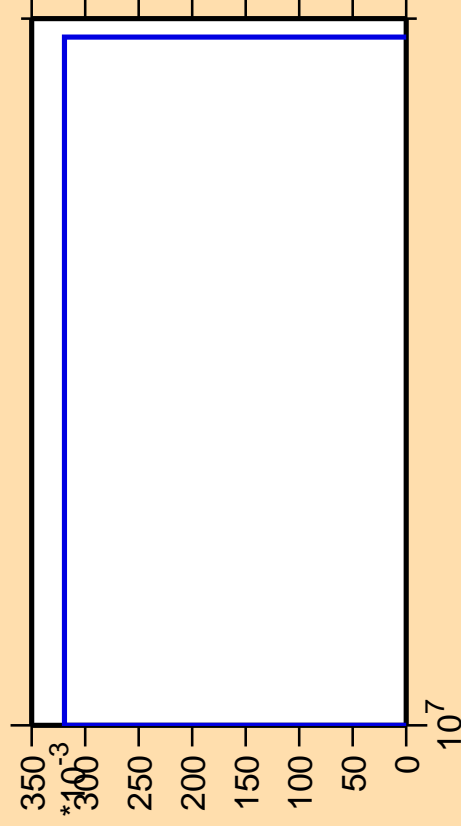
\Delta\sigma/\sigma vs. E for ^{198}\text{Tl} (mt 45)
