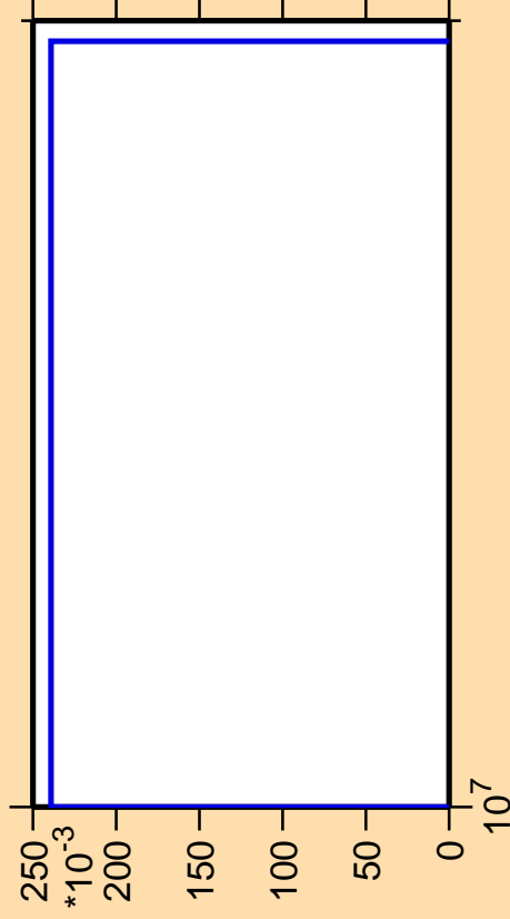
\Delta\sigma/\sigma vs. E for ^{198}\text{Tl}(\text{mt117})
