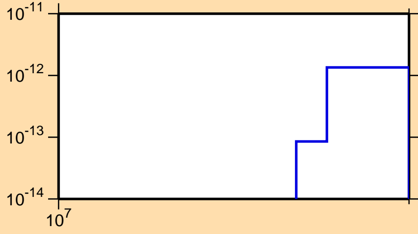
\sigma vs. E for ^{199}\text{Tl} (mt 45)
