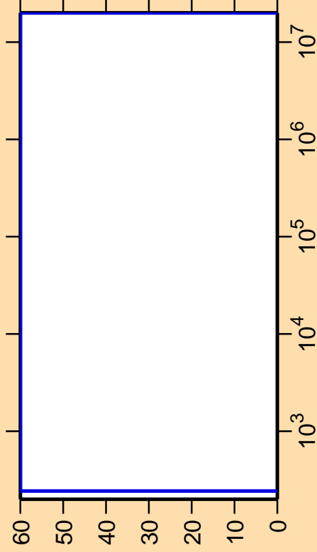
\Delta\sigma/\sigma vs. E for ^{199}\text{Tl}(n,\alpha)
