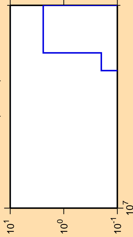
\Delta\sigma/\sigma vs. E for ^{199}\text{Tl}(\text{mt117})
