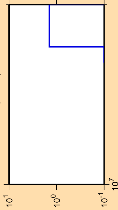
\Delta\sigma/\sigma vs. E for ^{199}\text{Tl} (mt 45)
