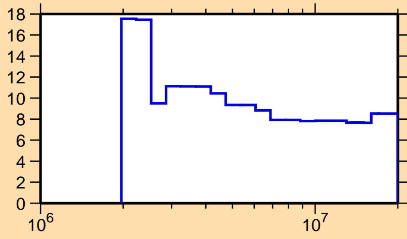
\Delta\sigma/\sigma vs. E for ^{199}\text{Tl}(n,n\text{onel.})
