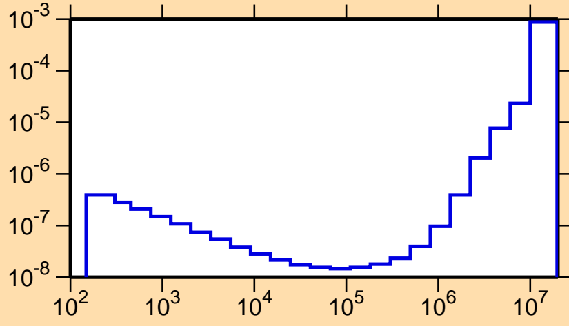
\sigma vs. E for ^{199}\text{Tl}(n,\alpha)
