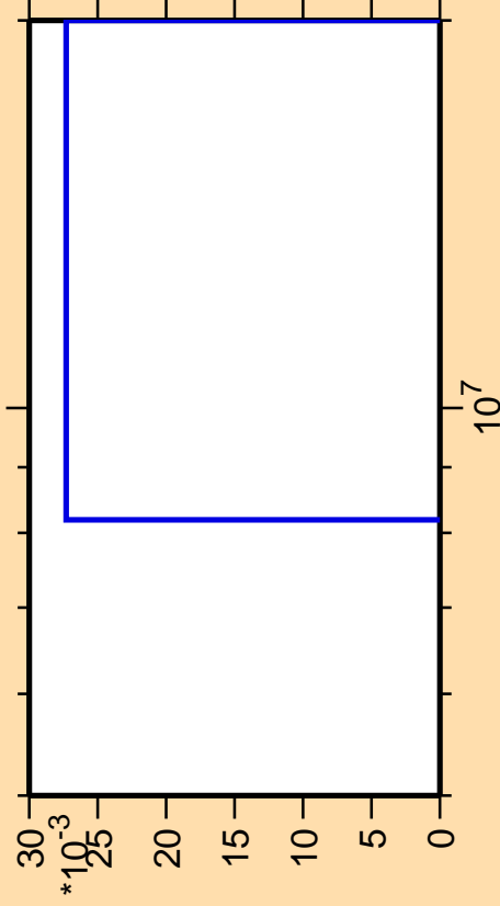
\Delta\sigma/\sigma vs. E for ^{199}\text{Tl}(\text{mt117})
