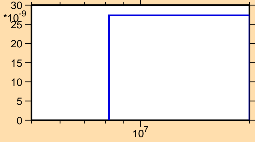
\sigma vs. E for ^{199}\text{Tl}(n,2np)
