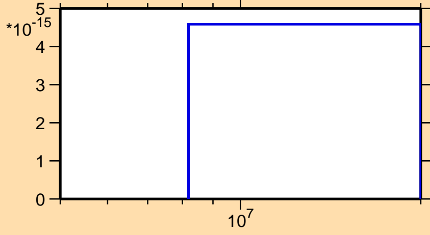
\sigma vs. E for ^{199}\text{Tl}(\text{mt117})
