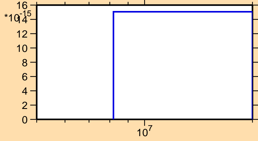
\sigma vs. E for ^{199}\text{Tl} (mt 45)
