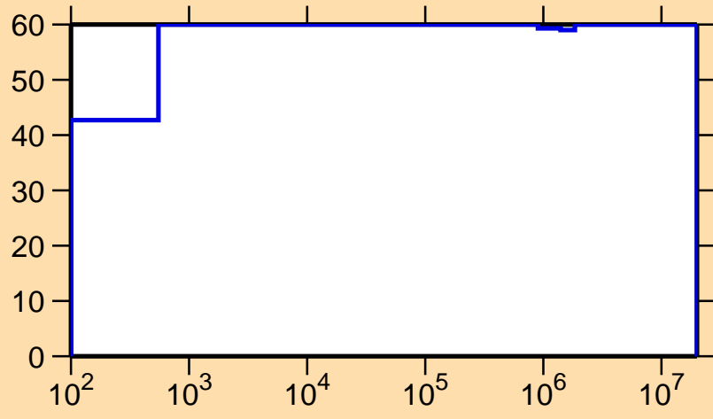
\Delta\sigma/\sigma vs. E for ^{199}\text{Tl}(n,\gamma)
