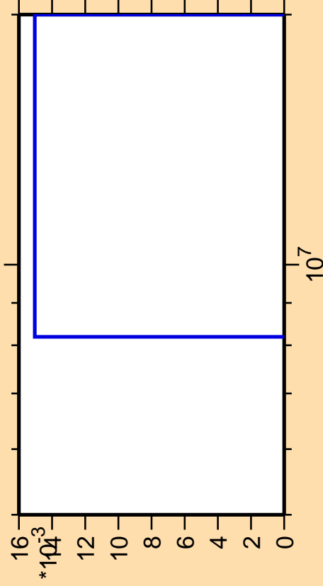
\Delta\sigma/\sigma vs. E for ^{199}\text{Tl} (mt 45)
