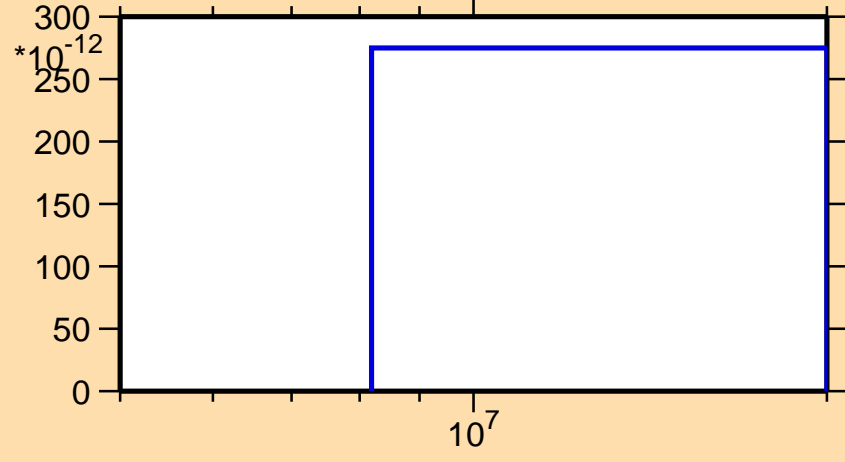
\sigma vs. E for ^{199}\text{Tl}(n,nt)
