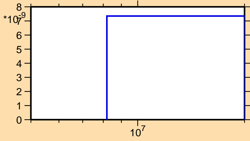
\sigma vs. E for ^{199}\text{Tl}(n,\text{nd})
