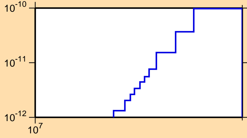
\sigma vs. E for ^{200}\text{Tl}(n,p\alpha)
