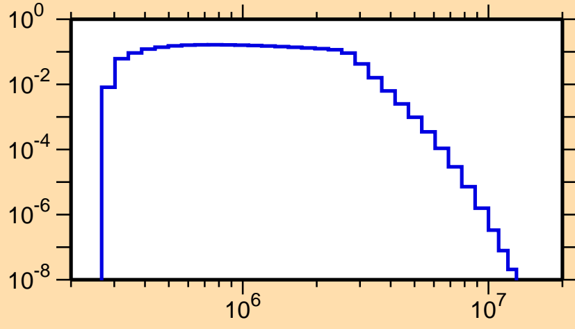
\sigma vs. E for ^{200}\text{Tl}(n,n_3)
