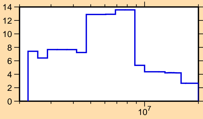
\Delta\sigma/\sigma vs. E for ^{200}\text{Tl}(n,\text{tot.})
