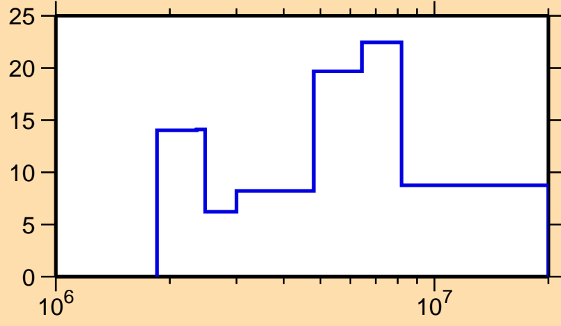
\Delta\sigma/\sigma vs. E for ^{200}\text{Tl}(n, el.)
