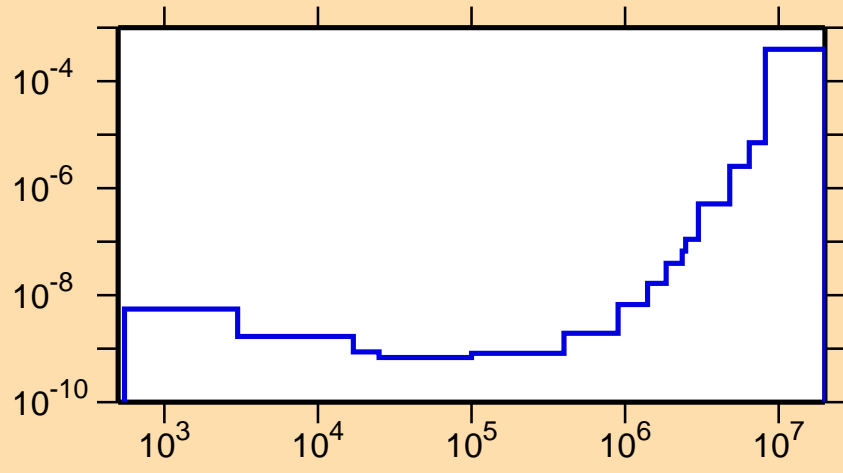
\sigma vs. E for ^{201}\text{Tl}(n,\alpha)
