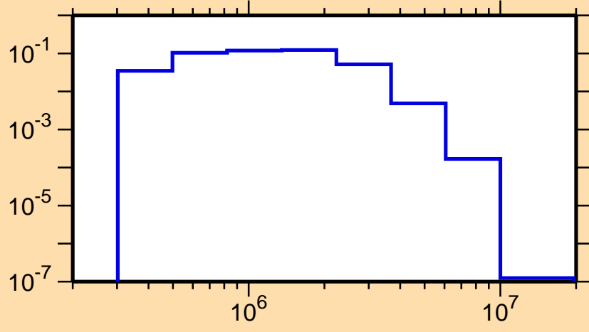
\sigma vs. E for ^{202}\text{Tl}(n,n_4)
