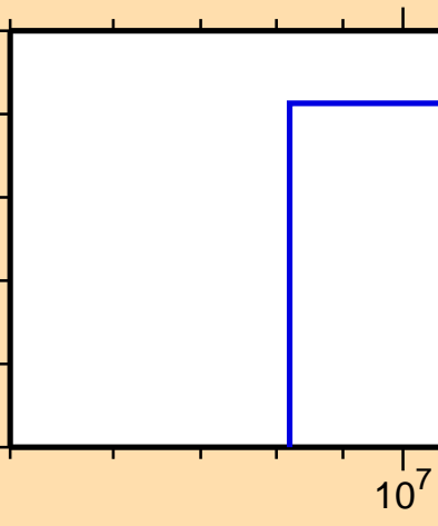
\sigma vs. E for ^{202}\text{Tl}(n,3n)
