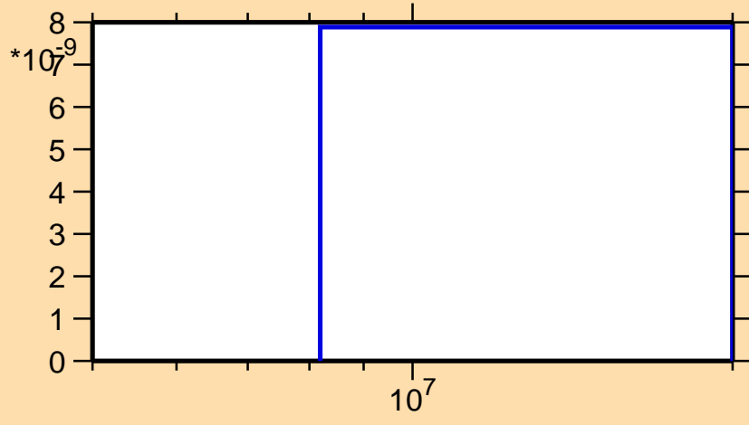
\sigma vs. E for ^{202}\text{Tl}(n,2n\alpha)
