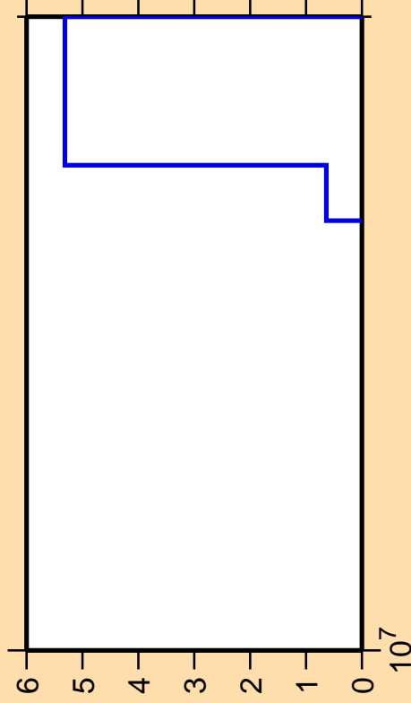
\Delta\sigma/\sigma vs. E for ^{203}\text{Tl}(n,p\alpha)
