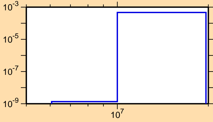
\sigma vs. E for ^{203}\text{Tl}(n,d)
