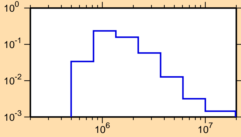
\sigma vs. E for ^{203}\text{Tl}(n,n_2)
