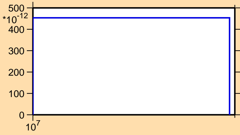
\sigma vs. E for ^{203}\text{Tl}(n,2np)
