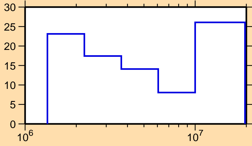
\Delta\sigma/\sigma vs. E for ^{203}\text{Tl}(n,ncont.)
