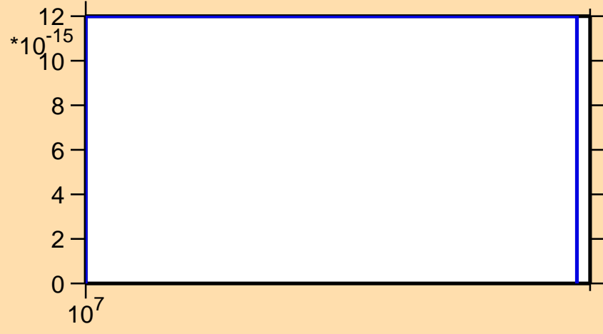
\sigma vs. E for ^{203}\text{Tl}(n,p\alpha)
