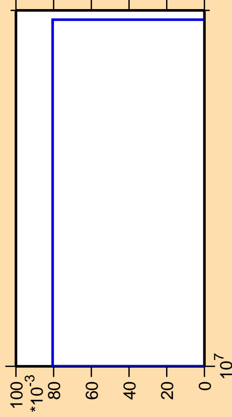
\Delta\sigma/\sigma vs. E for ^{203}\text{Tl}(n,p\alpha)
