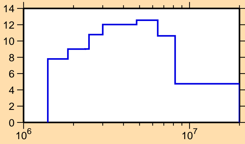
\Delta\sigma/\sigma vs. E for ^{203}\text{Tl}(n,el.)
