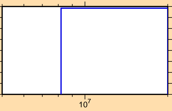
\sigma vs. E for ^{203}\text{Tl}(n,2n\alpha)
