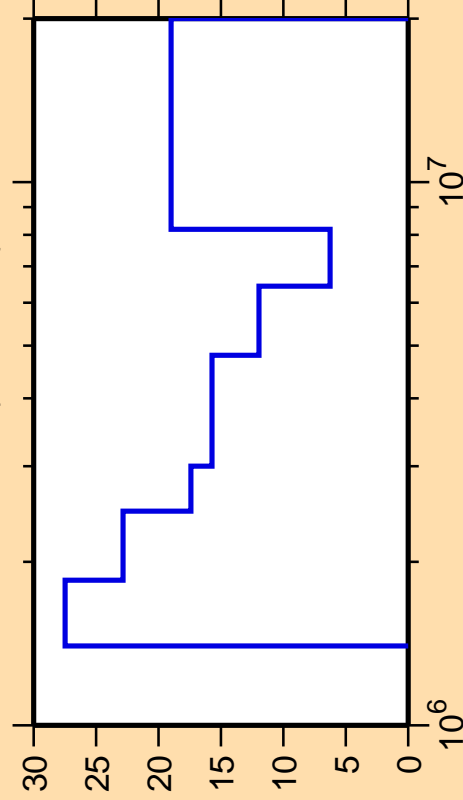
\Delta\sigma/\sigma vs. E for ^{203}\text{Tl}(n,\text{ncont.})
