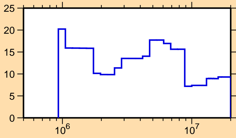
\Delta\sigma/\sigma vs. E for ^{204}\text{Tl}(n,el.)
