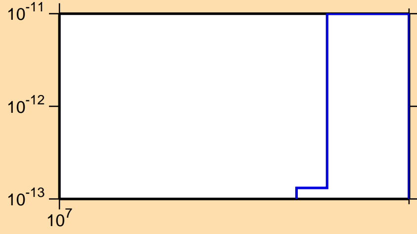
\sigma vs. E for ^{204}\text{Tl}(n,\text{He}3)
