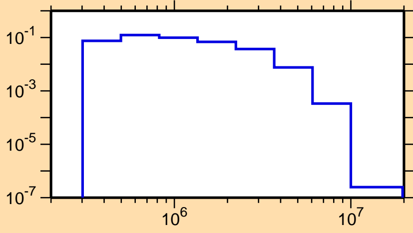
\sigma vs. E for ^{204}\text{Tl}(n,n_4)
