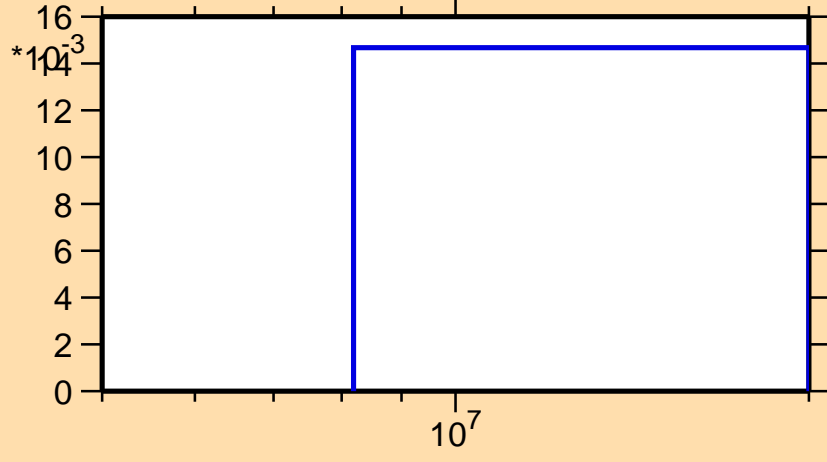
\sigma vs. E for ^{204}\text{Tl}(n,3n)
