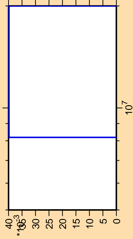
\Delta\sigma/\sigma vs. E for ^{204}\text{Tl}(n,p\alpha)
