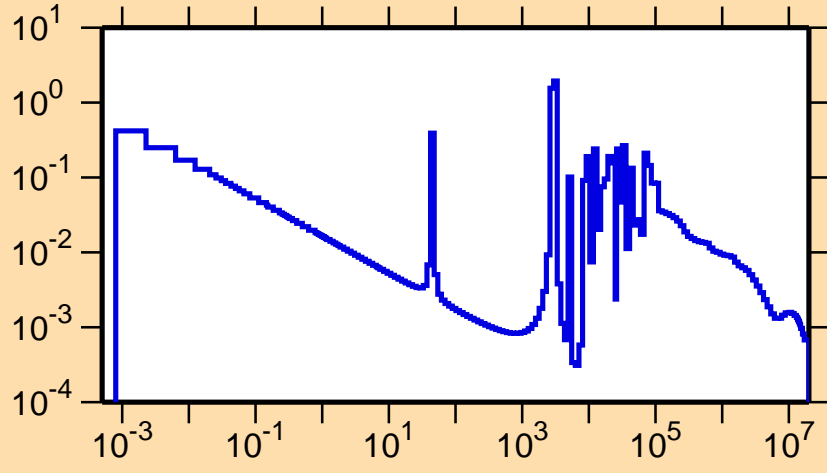
\sigma vs. E for ^{205}\text{Tl}(n,\gamma)
