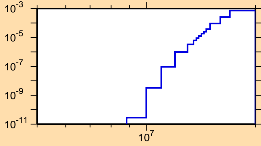
\sigma vs. E for ^{205}\text{Tl}(n,np)
