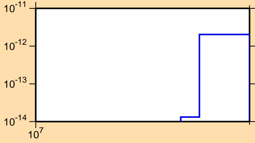
\sigma vs. E for ^{205}\text{Tl}(n,\text{He}3)
