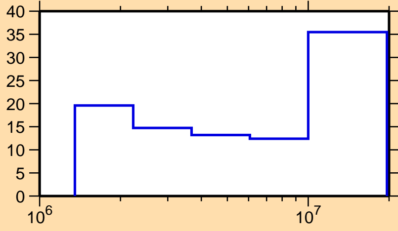
\Delta\sigma/\sigma vs. E for ^{205}\text{Tl}(n,n\text{cont.})
