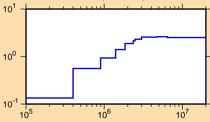
\sigma vs. E for ^{205}\text{Tl}(n,\text{nonel.})
