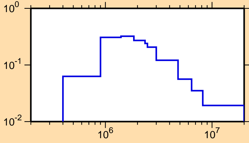
\sigma vs. E for ^{205}\text{Tl}(n,n_2)
