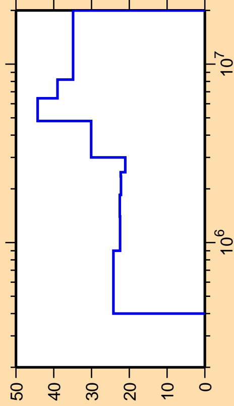
\Delta\sigma/\sigma vs. E for ^{205}\text{Tl}(n,n_2)
