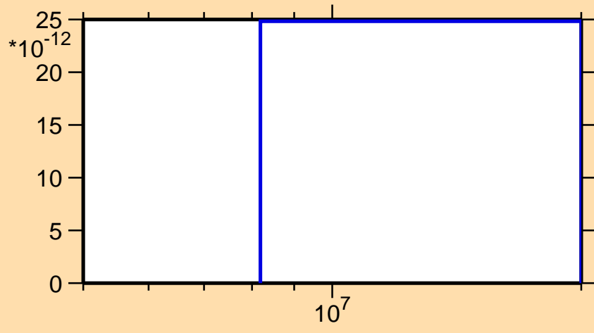
\sigma vs. E for ^{205}\text{Tl}(n,2np)
