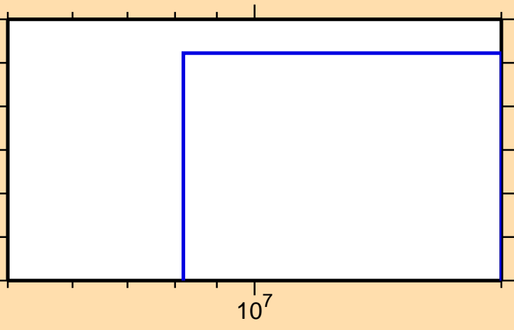
\sigma vs. E for ^{205}\text{Tl}(n,3n)
