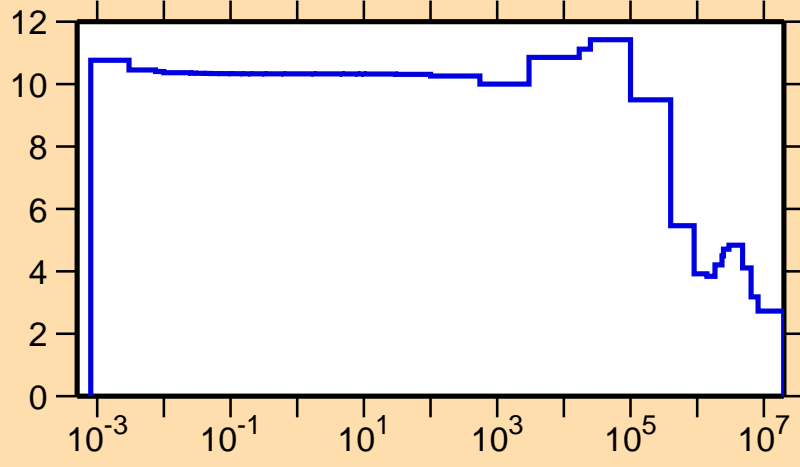
\sigma vs. E for ^{205}\text{Tl}(n,\text{el.})
