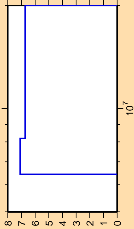
\Delta\sigma/\sigma vs. E for ^{206}\text{Tl}(n,n\text{cont.})
