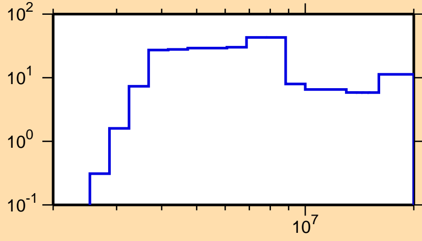
\Delta\sigma/\sigma vs. E for ^{206}\text{Tl}(n,p)
