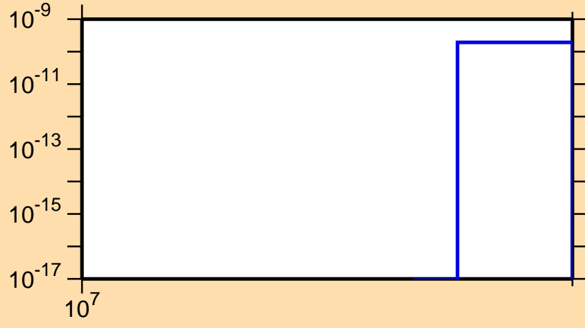
\sigma vs. E for ^{206}\text{Tl}(n,3n\alpha)
