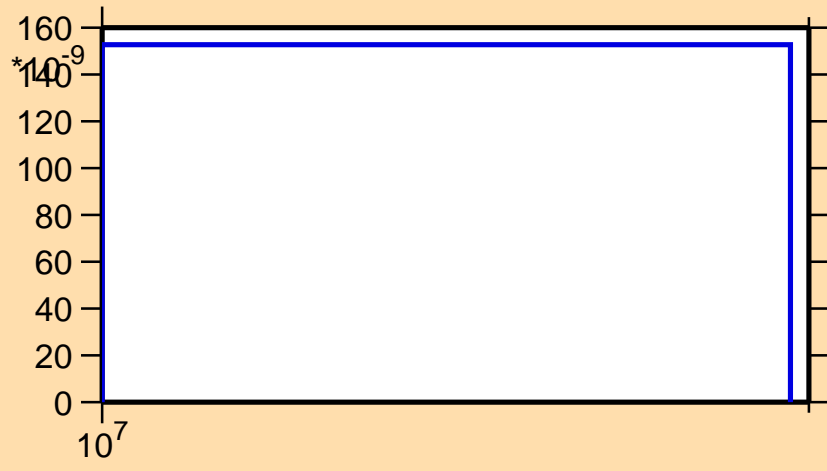
\sigma vs. E for ^{206}\text{Tl}(n,nd)
