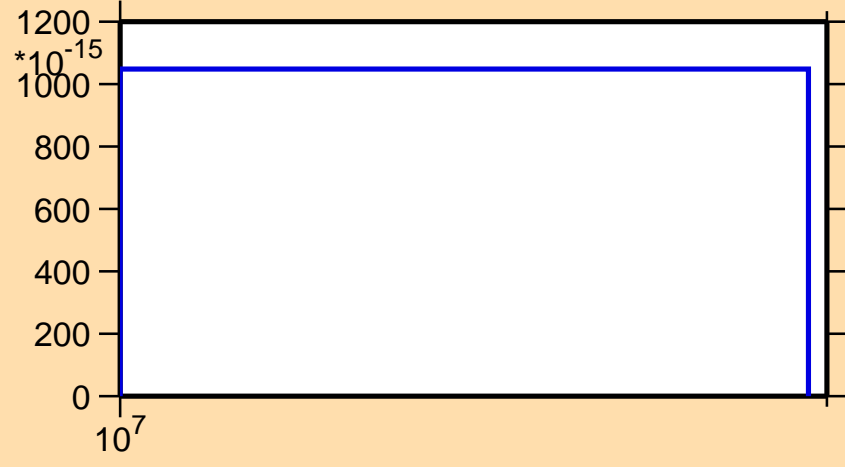
\sigma vs. E for ^{206}\text{Tl}(n,3n\alpha)
