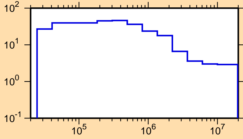
\Delta\sigma/\sigma vs. E for ^{206}\text{Tl}(n, n_{\text{nonel}})
