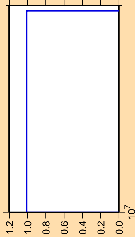
\Delta\sigma/\sigma vs. E for ^{206}\text{Tl}(n,3n\alpha)
