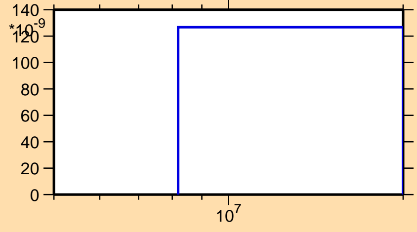
\sigma vs. E for ^{206}\text{Tl}(n,nd)
