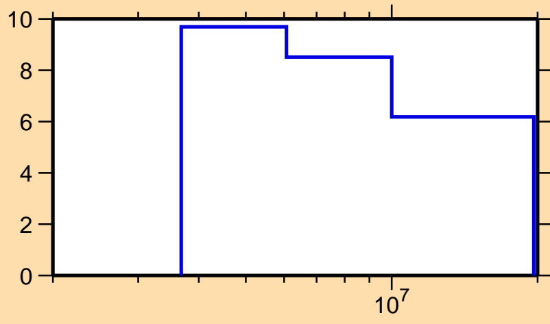
\Delta\sigma/\sigma vs. E for ^{207}\text{Tl}(n,n\text{nonel.})
