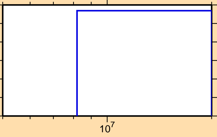
\sigma vs. E for ^{207}\text{Tl}(n,\text{nd})
