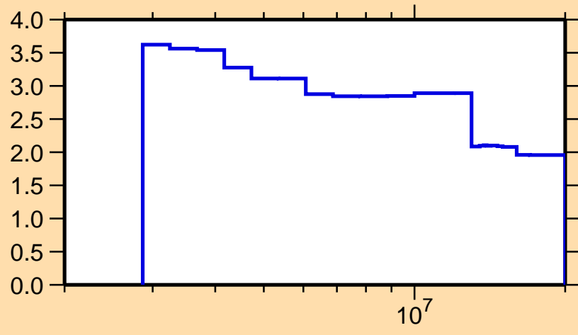
\Delta\sigma/\sigma vs. E for ^{207}\text{Tl}(n,n\text{onel.})
