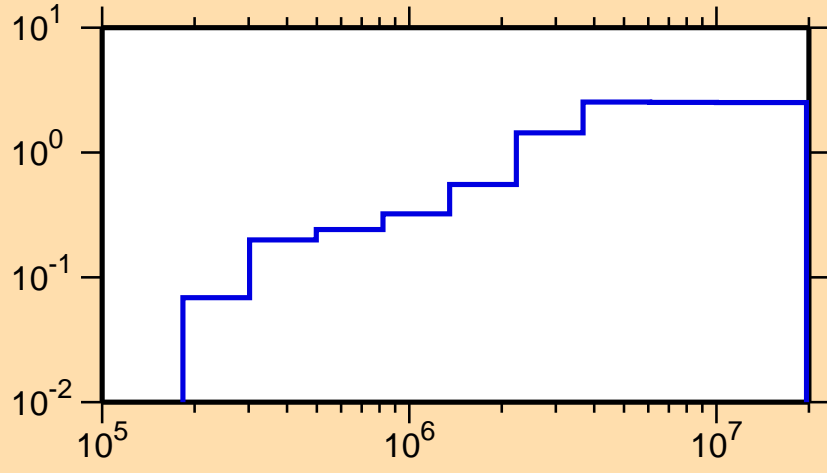
\sigma vs. E for ^{207}\text{Tl}(n,\text{nonel.})
