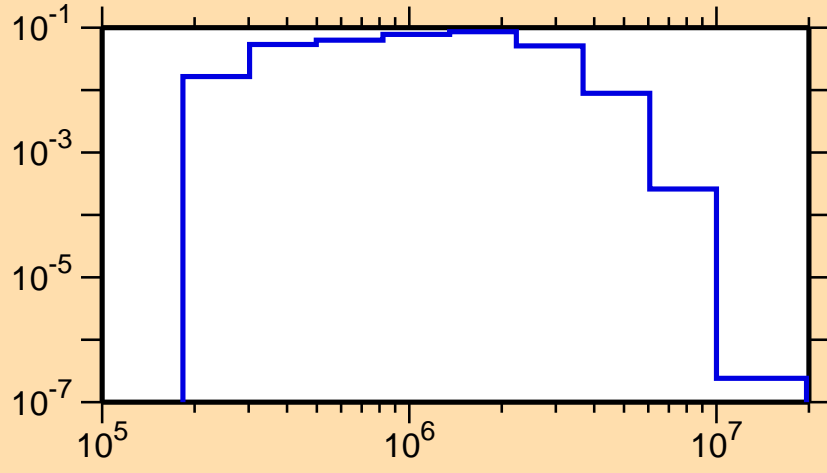
\sigma vs. E for ^{207}\text{Tl}(n,n_1)
