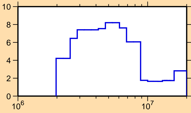
\Delta\sigma/\sigma vs. E for ^{208}\text{Tl}(n, el.)
