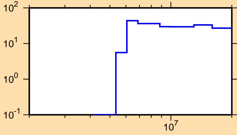
\Delta\sigma/\sigma vs. E for ^{208}\text{Tl}(n,p)
