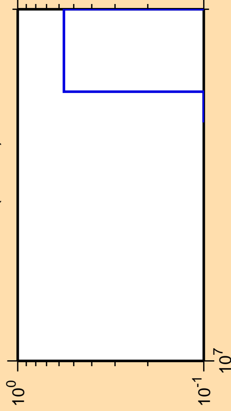
\Delta\sigma/\sigma vs. E for ^{208}\text{Tl}(n,3n\alpha)
